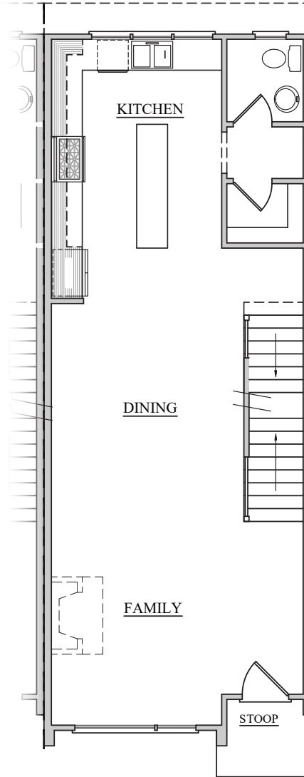
2ND FLOOR
